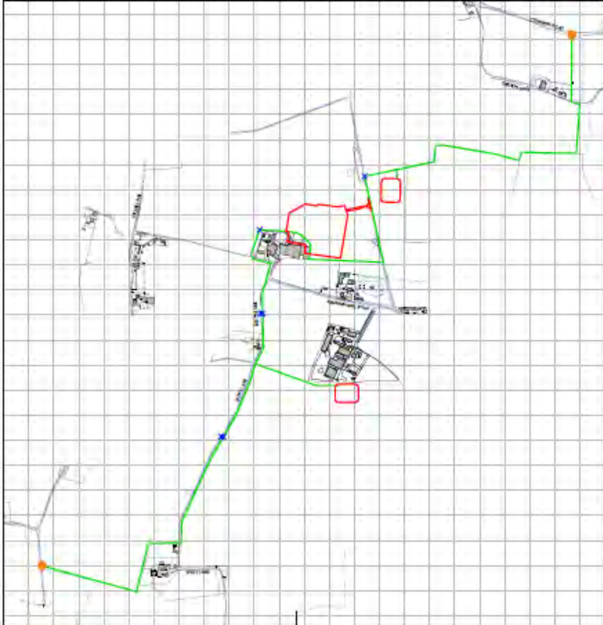
Figure 2.2 Application Red Line Boundary Showing Lagoon Locations and Digestate Pipeline Routes
