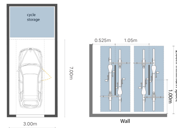
Figure 32: Illustrative layout of a garage with a cycle storage area (left), and illustrative layout for Sheffield cycle stands for visitors (right).
