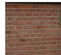
Figure 12: Stretcher bond
