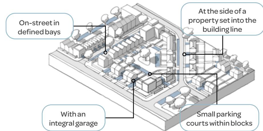
Parking options depend on the location and character of an area. A variety of arrangements can be used, ranging from integrated on-plot spaces, to successful parking courts.
