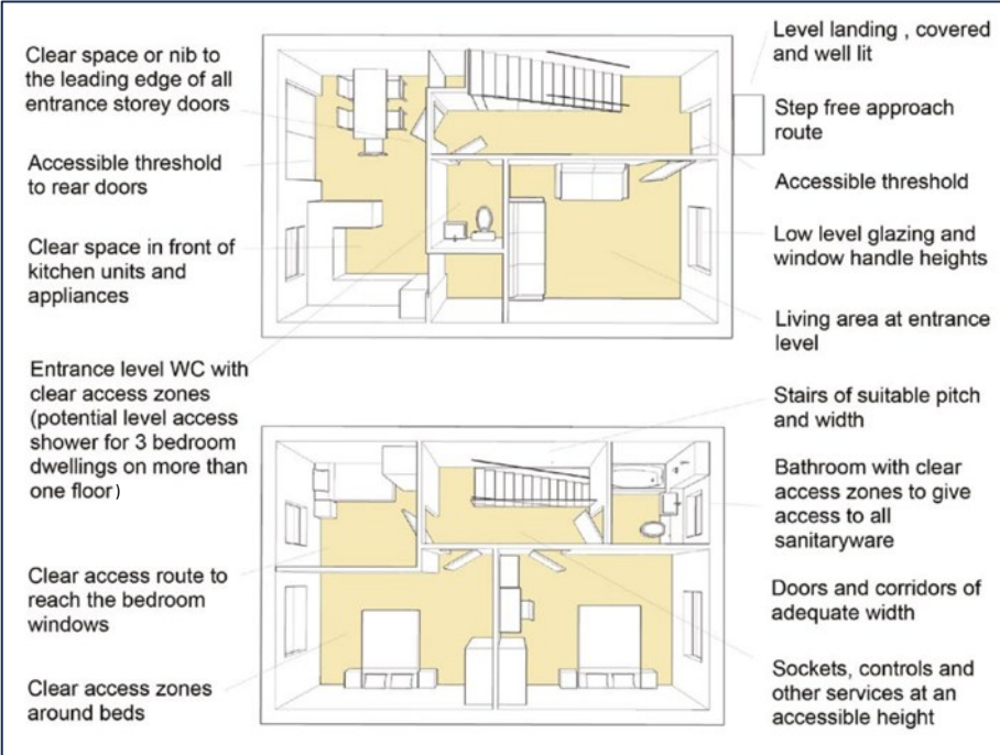
Figure 97: Pictorial example of a M4(2) Category 2 home. Source: Housing and disabled people – a toolkit for local authorities in England, planning for accessible homes, Equality and Human Rights Commission.
