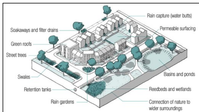
Figure 62: A variety of tools for sustainable drainage in different contexts. Source: National Model Design Code, Part 2, page 23.
