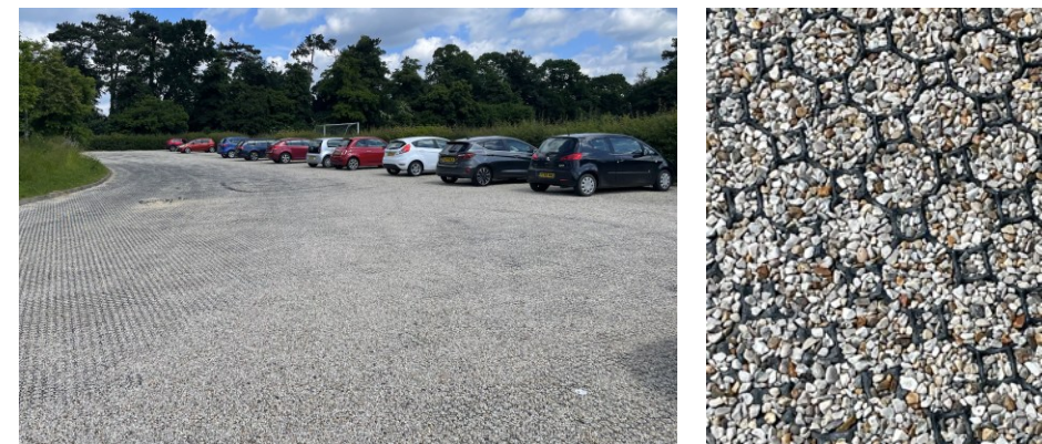
Figure 64: Permeable surfaced for car park. Community car park at Willow Centre, Cringleford, Norwich. Source: own.
